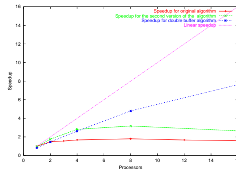
Figure 4 : Comparison between the scaling of the original parallel version and the new double buffer version
